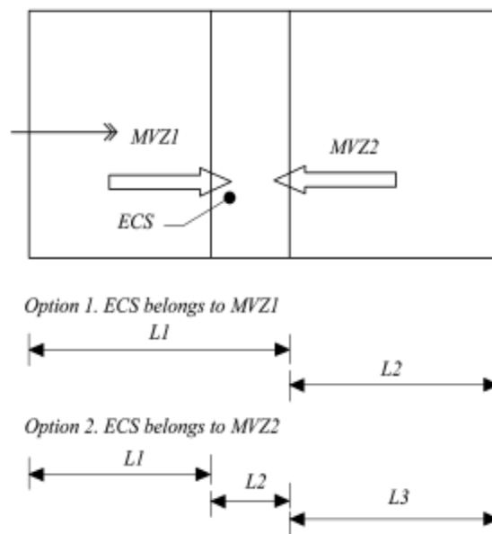
Fig. 2.2.1.2-4 ECS serves two MVZ
