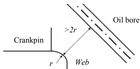
Fig. 2.1. Oil bore proximity to fillet
