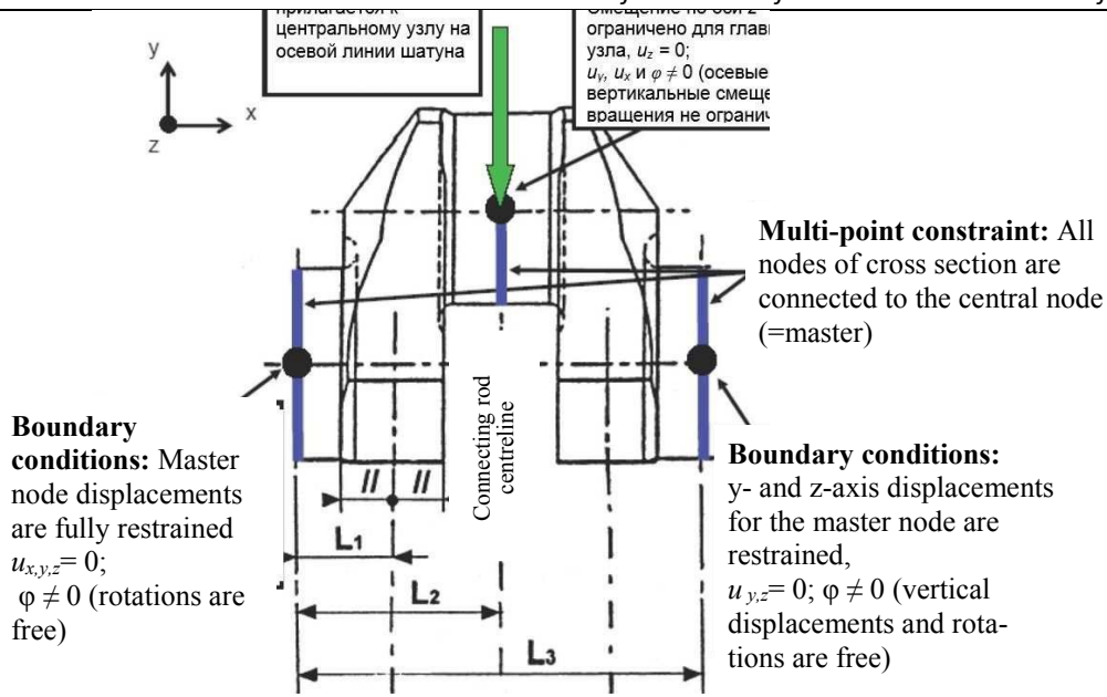
Fig. 3.3. Boundary and load conditions for 3-point bending load case of in-line engine
