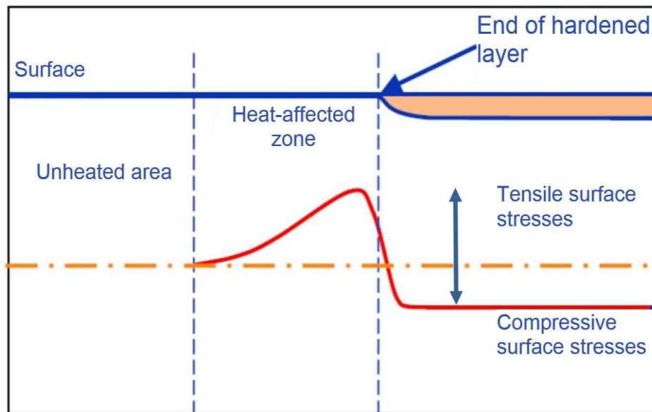
Fig. 4-2. Residual stresses along the surface of a crankpin and fillet
