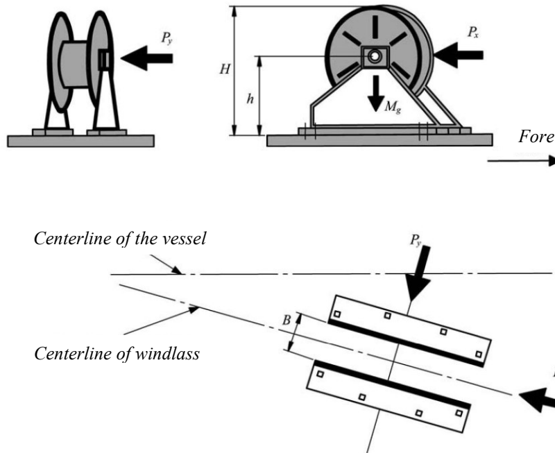
Fig. 6.3.5.3 Direction of forces
