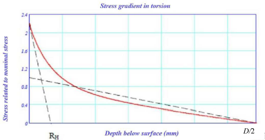
Fig. 3.1-2. Torsional SCF in crankpin fillet as a function of depth. The corresponding SCF for the journal fillet can be found by replacing R_H with R_G and D with D_G
