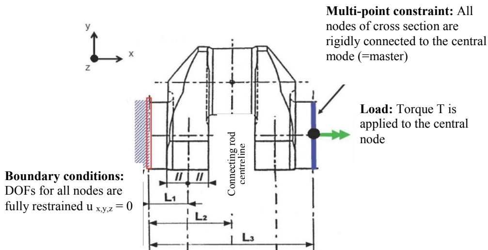
Fig. 3.1. Boundary and load conditions for torsion load case
