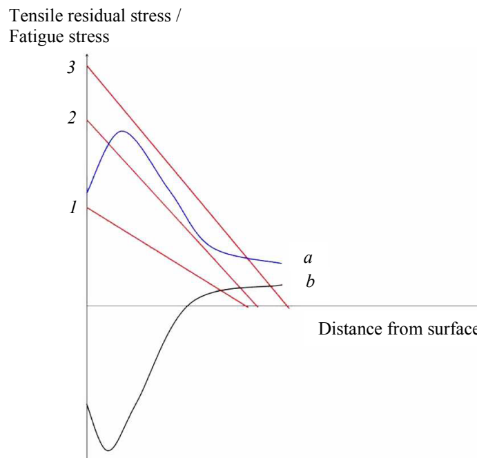
Fig. 6.1. Working and residual stresses below the stroke-peened surface. Straight lines 1 to 3 represent different possible load stress gradients Gradiented load (e.g. bending and torsion) 1. Fatigue strength - without hairline cracks 2. Non-propagable hairline crack 3. Fatigue strength - rupture level a. Fatigue strength (total of residual stress and base fatigue strength of quenched and tempered material) b. Residual stress after peening.
