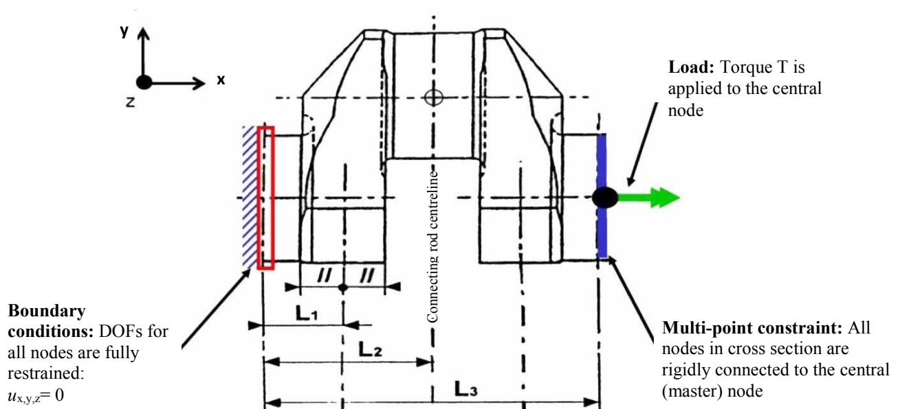
Fig. 3.1. Boundary and load conditions for torsion load case
