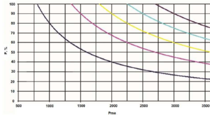
Fig. 2.11.3.2. Maximum possible sudden power increases as a function of brake mean effective pressure, P_{me} , at declared power (four-stroke diesel engines: P_{me} – declared power mean effective pressure (in kPa); P – power increase referred to declared power at site conditions; 1 – first power stage; 2 – second power stage; 3 – third power stage; 4 – fourth power stage; 5 – fifth power stage).
