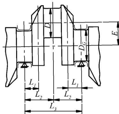
Fig.2.4.4.1-1. Crank throw for in-line engine
