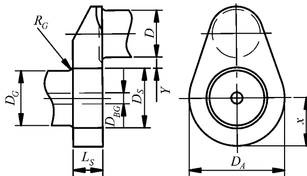
Fig.2.4.10.1. Crank throw of semi-built crankshaft:
