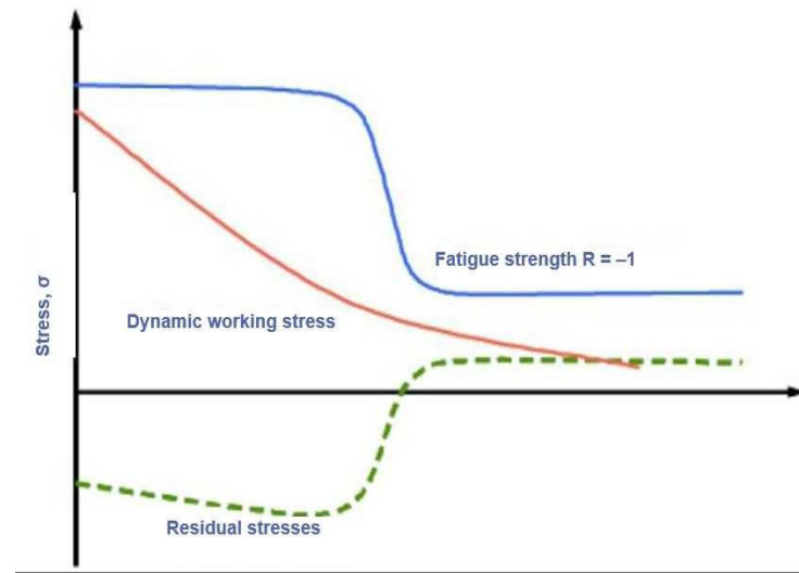
Fig. 3. . Stresses as functions of depth, general principles
