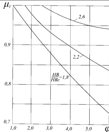
Fig. 4.2.2.8. 8 Diagram for determining the factor \mu_T versus \varphi and HB/HBc
