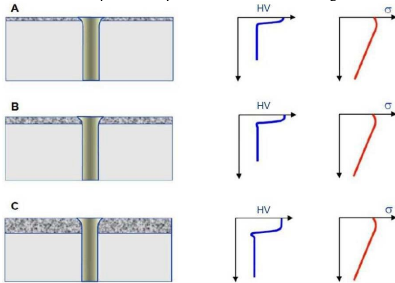
Fig. 3.2. Stresses and hardness in induction hardened oil hole outlets
