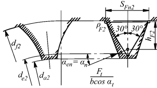
Fig.4.2.2.7.3.2-4. Illustration to the definition of Y_F for internal tooth
