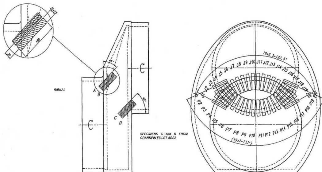
Fig. 3. Specimen locations in a crank throw
