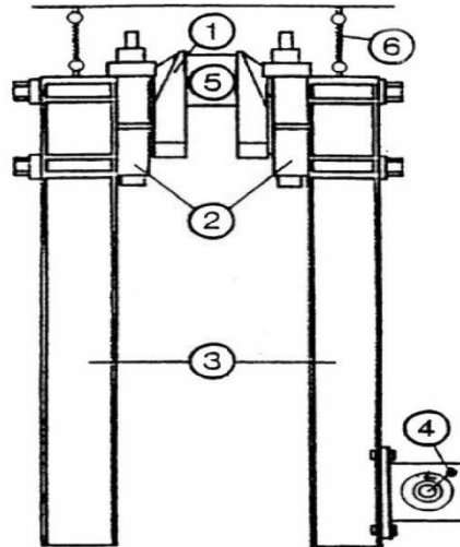
Fig. 4.2-1. An example of resonance test rig setup for bending loading test 1 — Crank throw; 2 — Mounts; 3 — "I" beam; 4 — Eccentric driven by speed-controlled motor; 5 — Strain gauge to adjust and monitor loading; 6 — Elastic suspension
