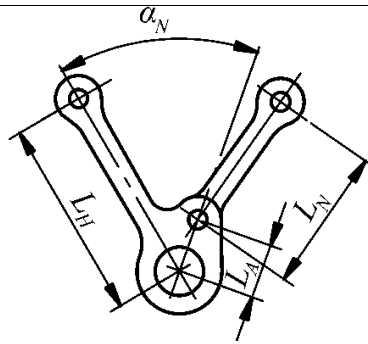
Fig.2.4.3-2. Articulated-type connecting rod
