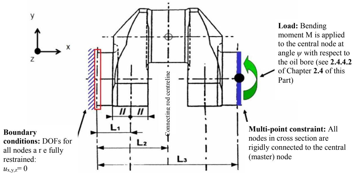
Fig. 3.2. Boundary and load conditions for pure bending load case
