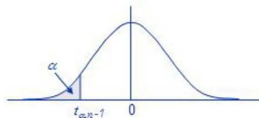
Fig. 2.5. Student's distribution
