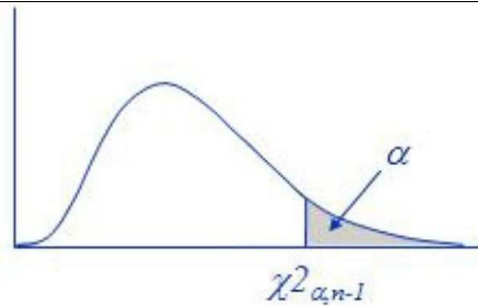
Fig. 2.6. Chi-square distribution
