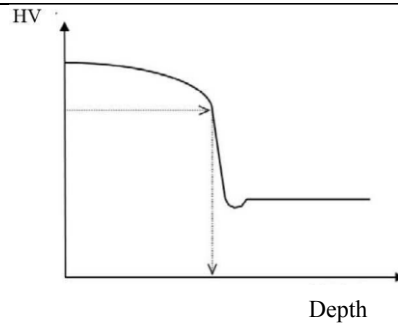
Fig. 4-1. Typical hardness as a function of depth. The arrows indicate the hardening depth
