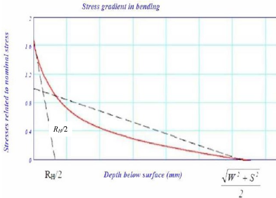
Fig. 3.1-1. Bending SCF in crankpin fillet as a function of depth. The corresponding SCF for the journal fillet can be found by replacing R_H with R_G
