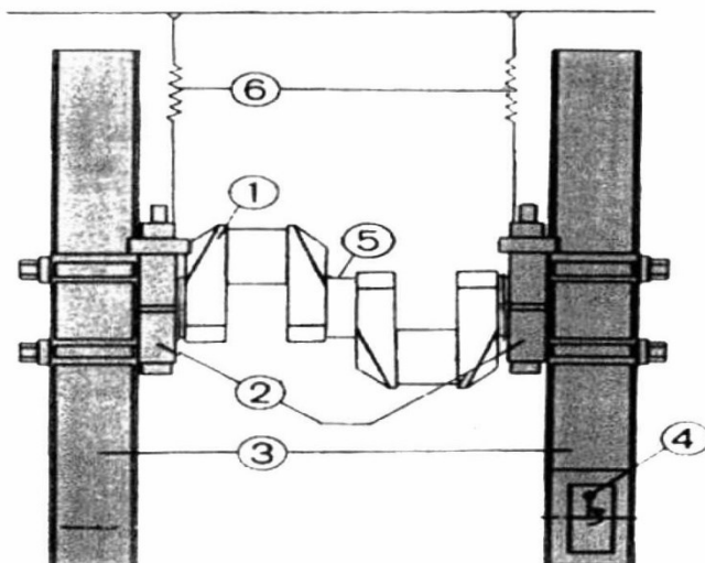
Fig. 4.2-2. An example of testing arrangement of the resonance tester for torsion loading with double crank throw section 1 — Crank throw; 2 — Clamp; 3 — I-beams; 4 — Motor-driven eccentric weight; 5 — Strain gage; 6 — Elastic suspension
